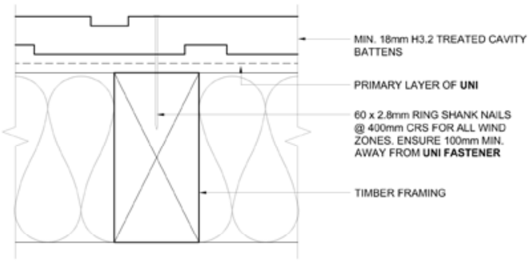
HORIZONTAL CAVITY BATTEN
