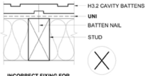
INCORRECT FIXING FOR VENTILATED BATTENS
